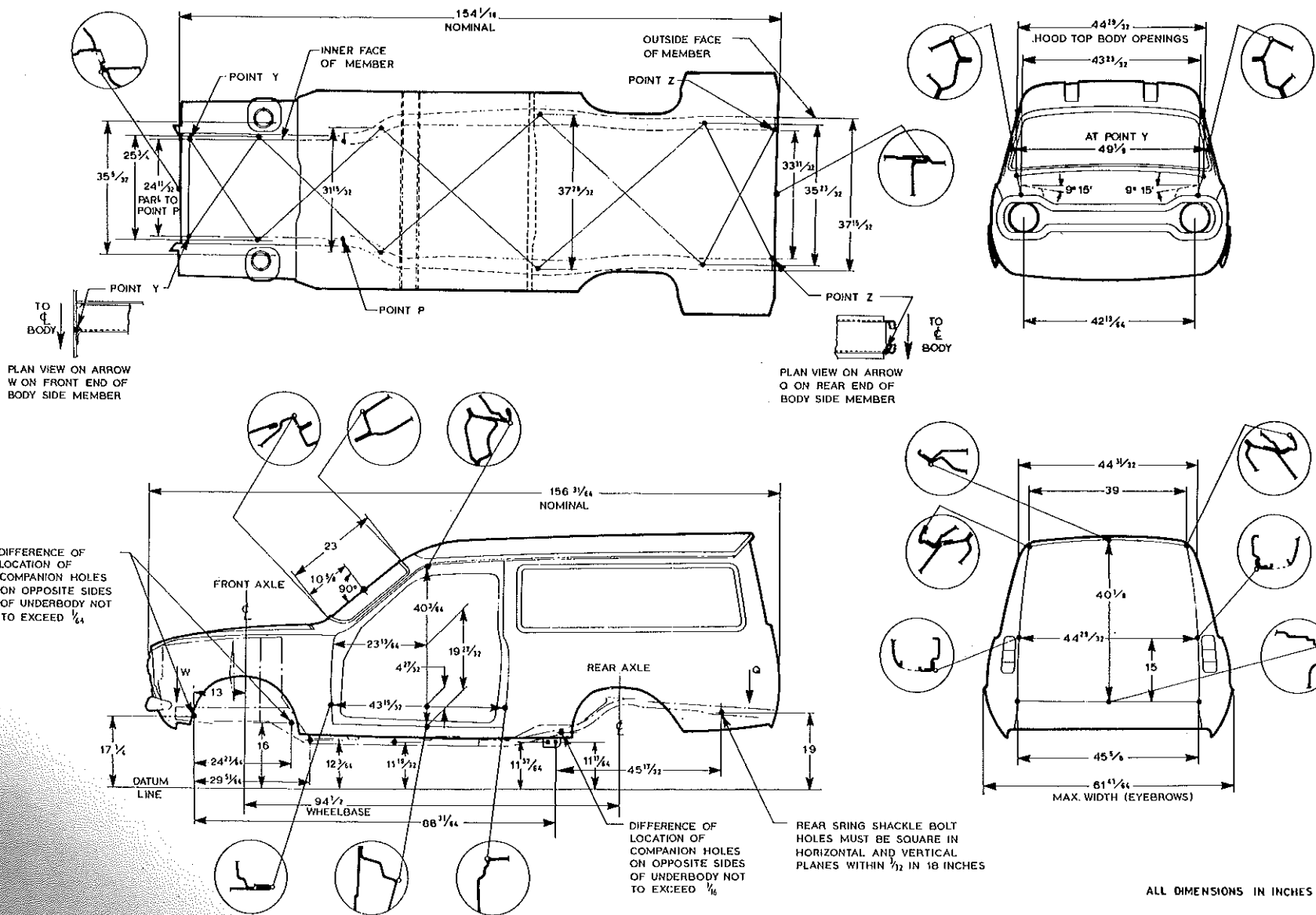
BODY TOLERANCE CHART—VAN
